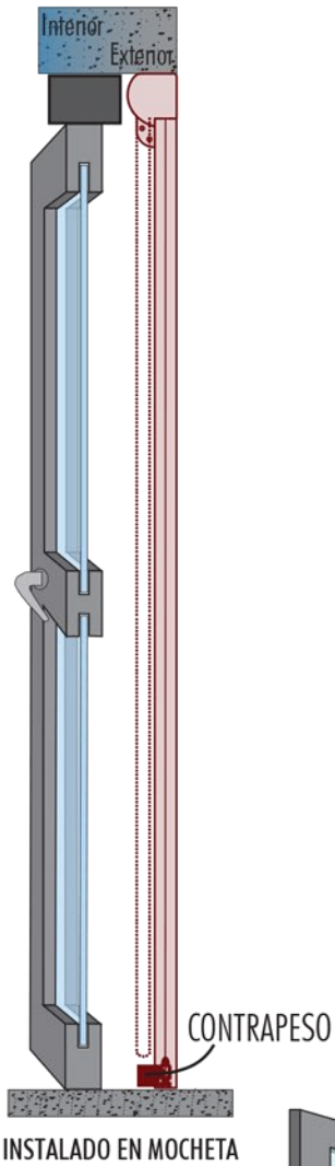
CORTE VERTICAL
