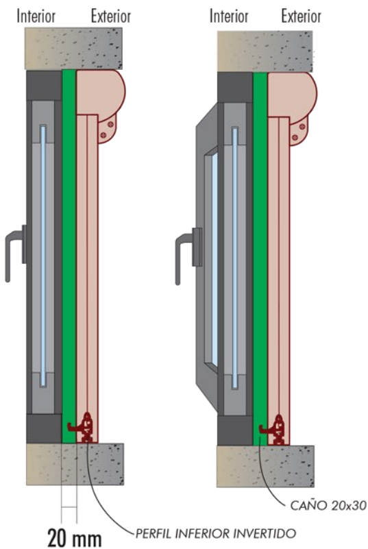
CORTE VERTICAL
